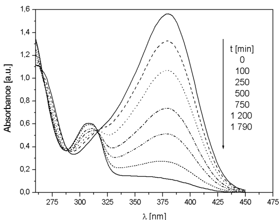
Figure 8a. Change of UV-VIS spectra during reaction kin3 in methanol ( t = 40^\circ ; c_{\text{cat}} = 5 \times 10^{-4} \text{ mol} \cdot \text{dm}^{-3} ).
