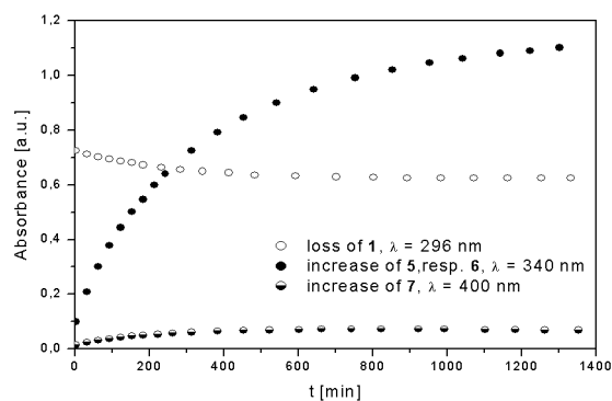
Figure 5a. Time change of absorbance during reaction kin1 in 2-propanol at 40°.
