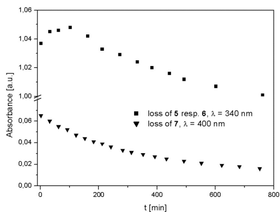
Figure 6. Time change of absorbance during reaction kin2 in 2-propanol at 40°.
