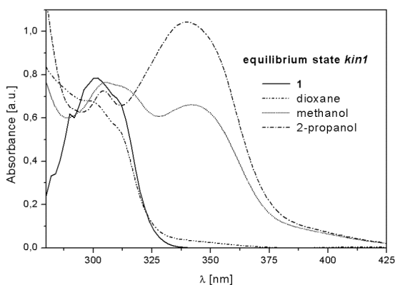
Figure 3. UV-VIS spectra of equilibrium states kin1 in various solvents and of aldehyde.
